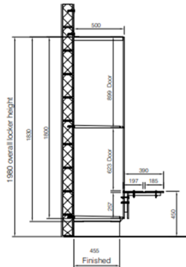
section detail welled locker with cantilevered bench
