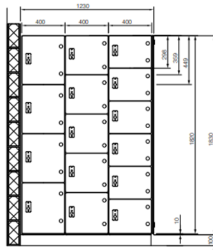
generic locker front elevation 400mm wide
