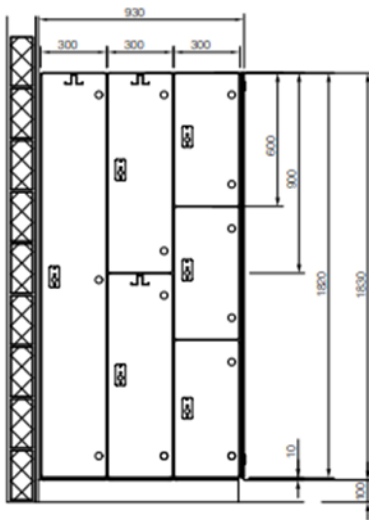
generic locker front elevation 300mm wide
