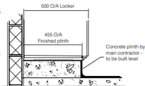
concrete plinth option
