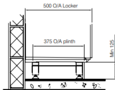
aluminium frame plinth option
