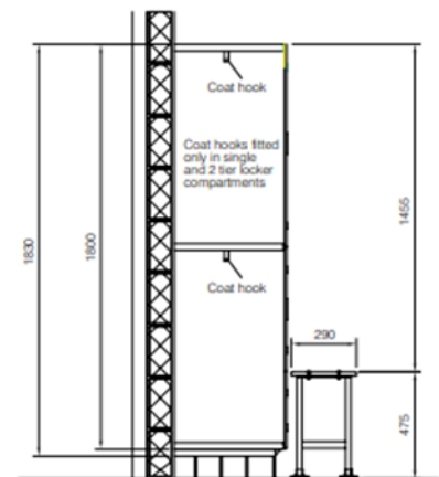
section detail welled locker with floor mounted bench
