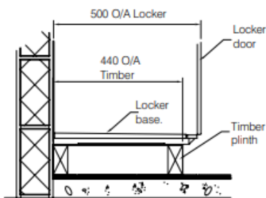
timber plinth option
