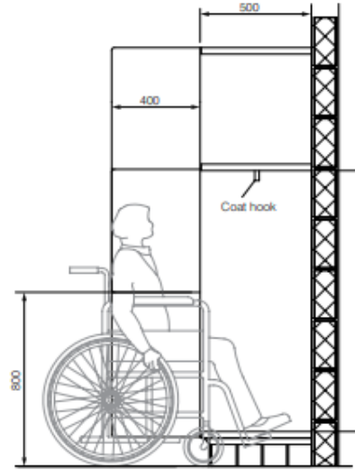
accessible lockers section
