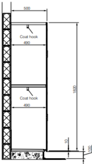
generic locker side elevation
