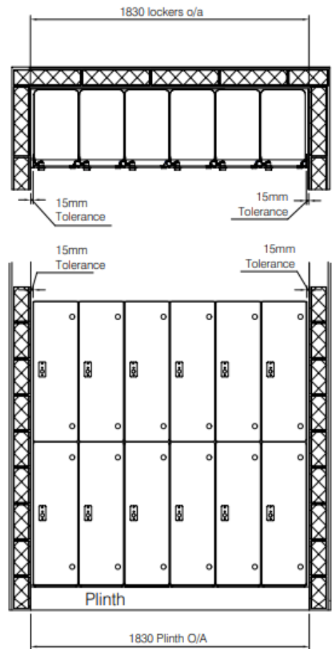
locker tolerance between walls
