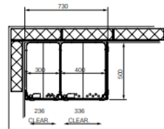
locker plan clear opening size for 300mm & 400mm wide 'Z' locker
