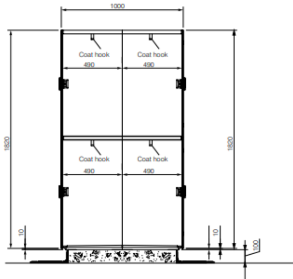
back to back lockers side elevation
