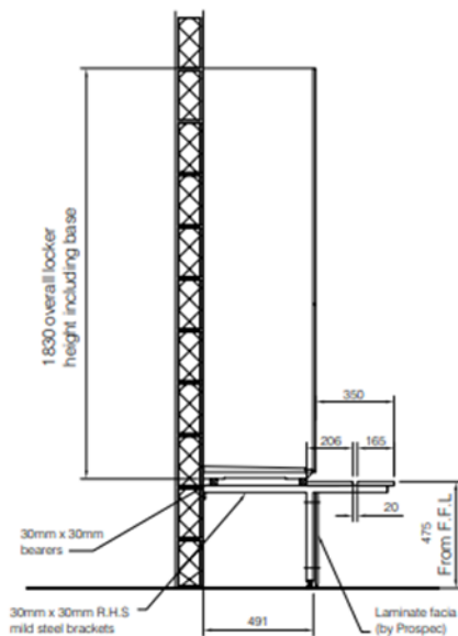
section detail locker support bench seating
