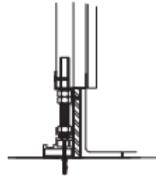
plinth detail 9mm WBP ply to tile & render
