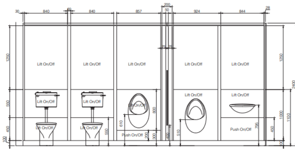
front elevation
